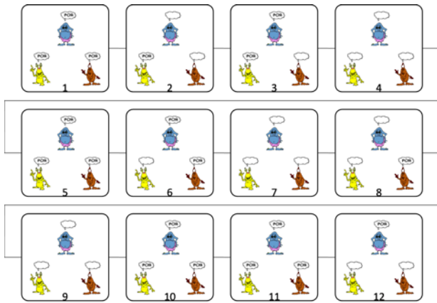
Figure 2: An example of a pattern set presented in Experiment 1. For each of these sets subjects were requested to choose the causal structure that presumably generated the data.
